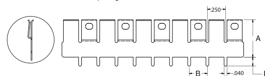
FIGURE 6 .25" Pin Spacing, No Standoff
