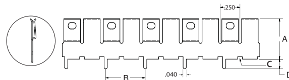
FIGURE 3 .25" Pin Spacing
