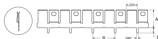
FIGURE 3 1.0" Pin Spacing, No Standoff
