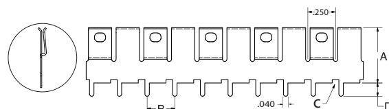
FIGURE 3 .25" Pin Spacing
