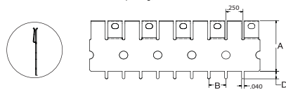
FIGURE 8 .25" Pin Spacing, No Standoff
