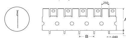
FIGURE 3 .50" Pin Spacing, No Standoff, No Holes
