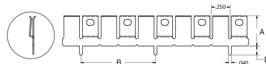
FIGURE 4 1.0" Pin Spacing, With Standoff
