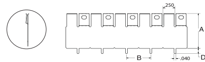
FIGURE 4 .50" Pin Spacing, With Standoff
