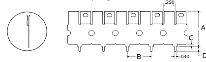
FIGURE 5 1.0" Pin Spacing, No Standoff, With Holes
