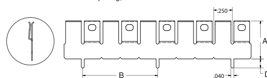
FIGURE 5 1.0" Pin Spacing, With Standoff
