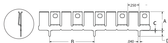
FIGURE 5 .25" Pin Spacing, No Standoff
