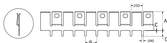
FIGURE 6 .25" Pin Spacing, With Standoff
