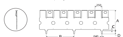
FIGURE 7 1.0" Pin Spacing, With Standoff, with holes
